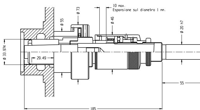
Expanding burnishing tool
