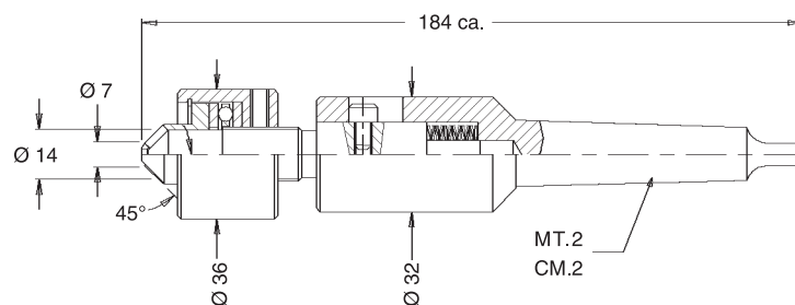
Internal conical burnishing tool
