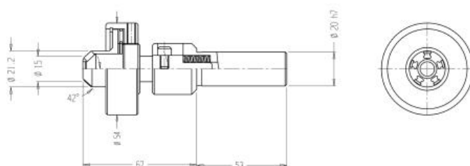
Internal conical burnishing tool
